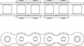
Chain-6 pitches long, including connecting link.
