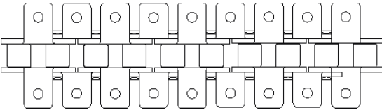
Chain-9 pitches long, with bent attachments, both sides of chain, every pitch.
