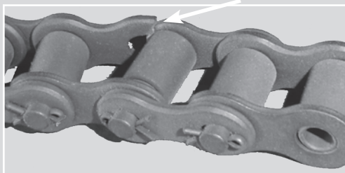
Roller Link Plate Tensile Failure
