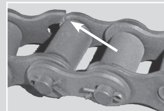
Roller Link Plate Tensile Failure
