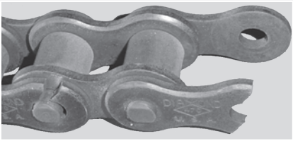
Pin Link Plate Fatigue Failure
