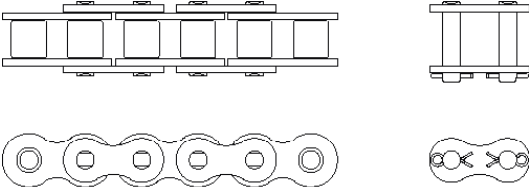
Chain-24 pitches long, riveted endless.
