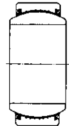
SAR1··SS with seal
